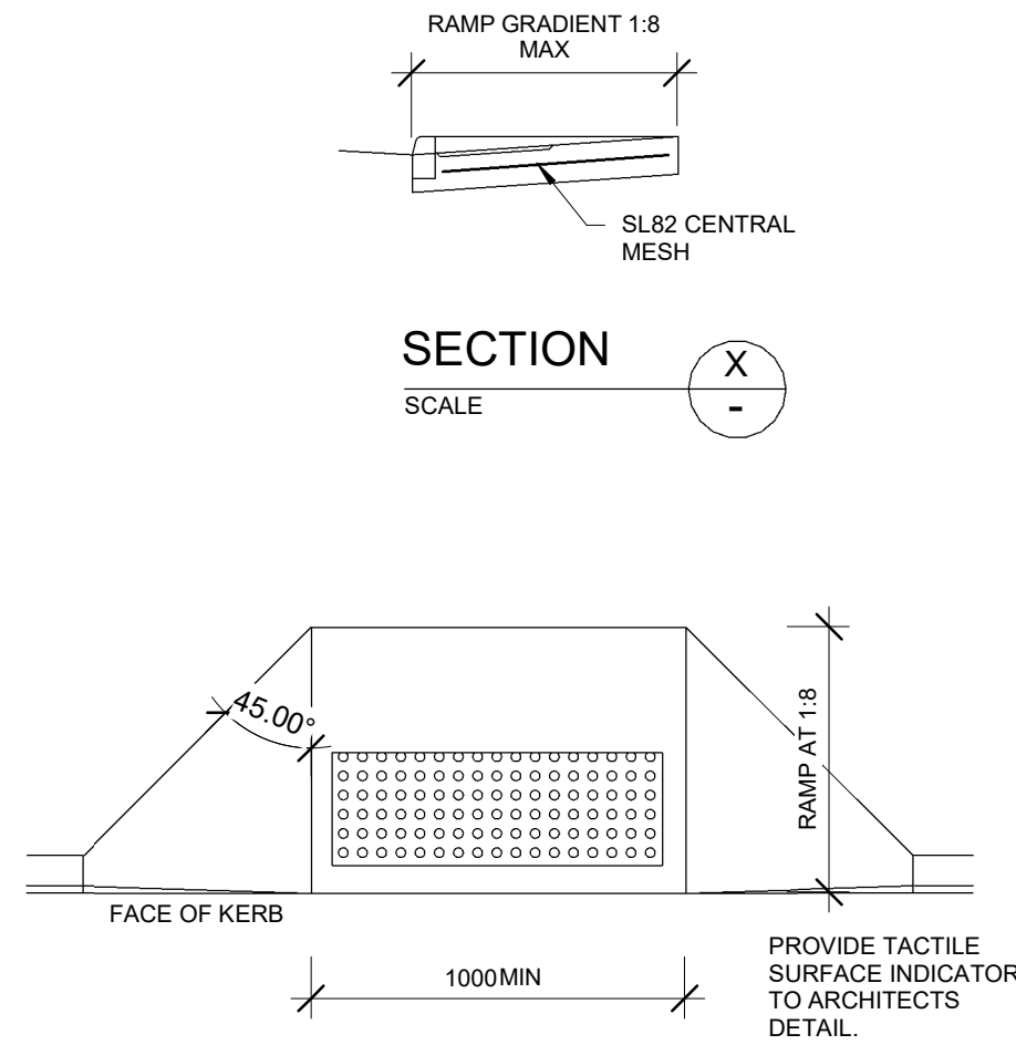
PRAM RAMP - PLAN Scale 1:20
