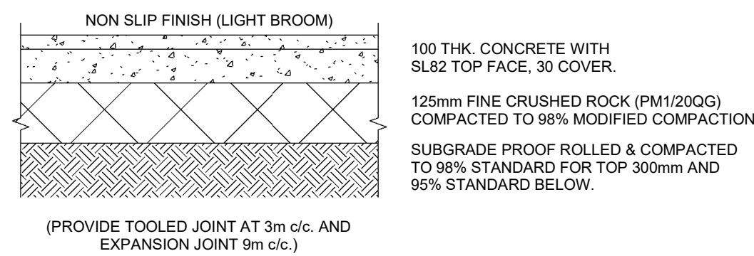
CONCRETE PAVEMENT - LIGHT DUTY (PEDESTRIAN PAVING) Scale 1:10
