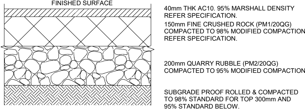
ASHALT PAVEMENT - HEAVY DUTY (REFER SPECIFICATIONS AND PLANS) Scale 1:10
