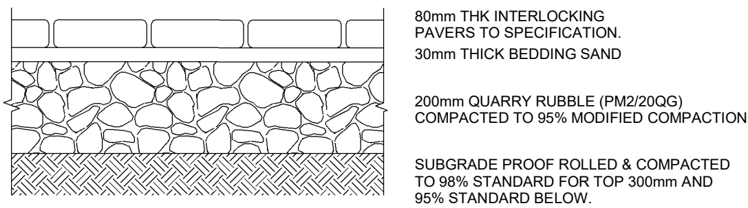
MASONRY PAVEMENT - MEDIUM DUTY (CARPARK PAVING) Scale 1:10
