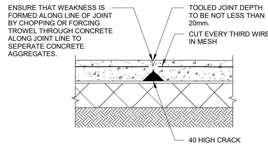
TOOLED JOINT DETAIL Scale 1:10
