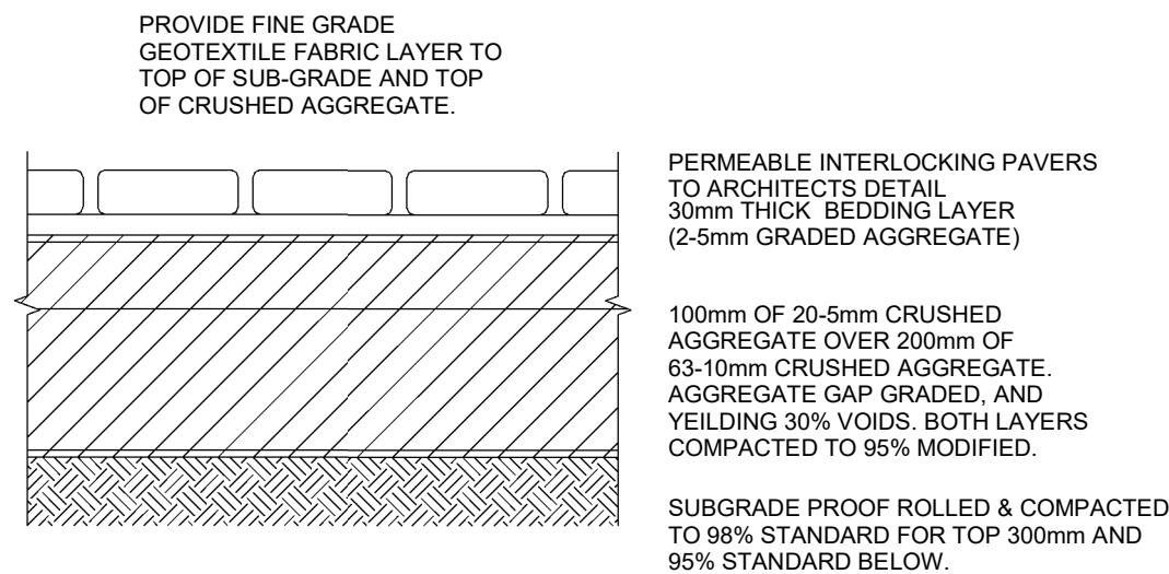
PERMEABLE PAVEMENT DETAIL Scale 1:10
