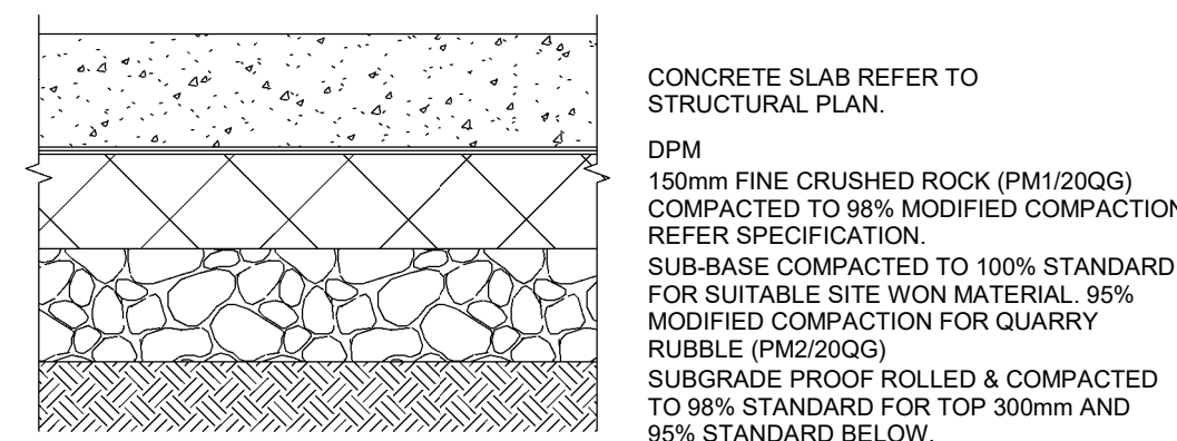
BUILDING PLATFORM Scale 1:10
