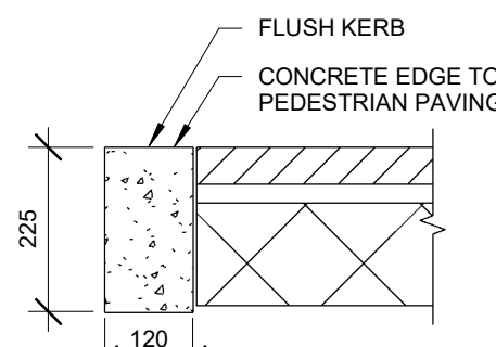
FLUSH KERB Scale 1:10
