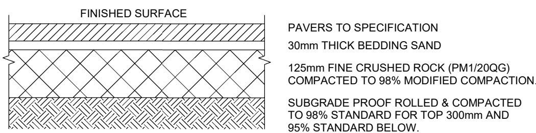
MASONRY PAVEMENT - LIGHT DUTY (PEDESTRIAN PAVING) Scale 1:10
