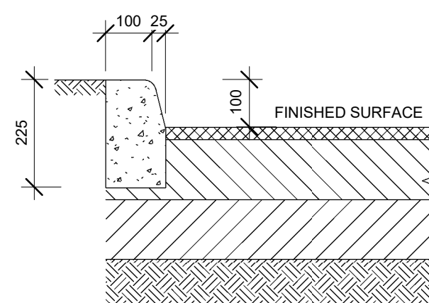
100 HIGH KERB Scale 1:10
