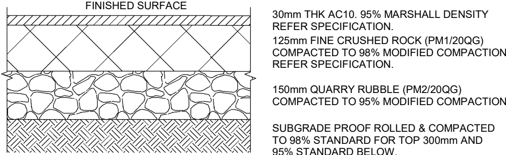
ASHALT PAVEMENT - MEDIUM DUTY (CARPARK PAVING) Scale 1:10
