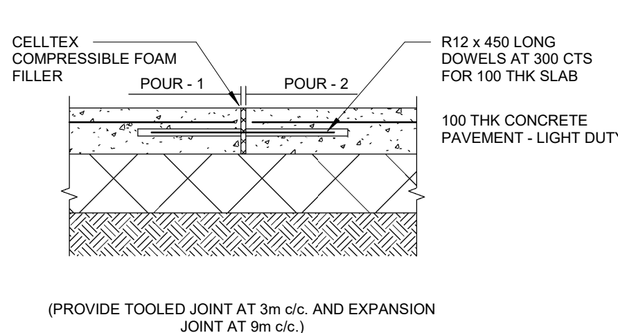
EXPANSION JOINT DETAIL Scale 1:10
