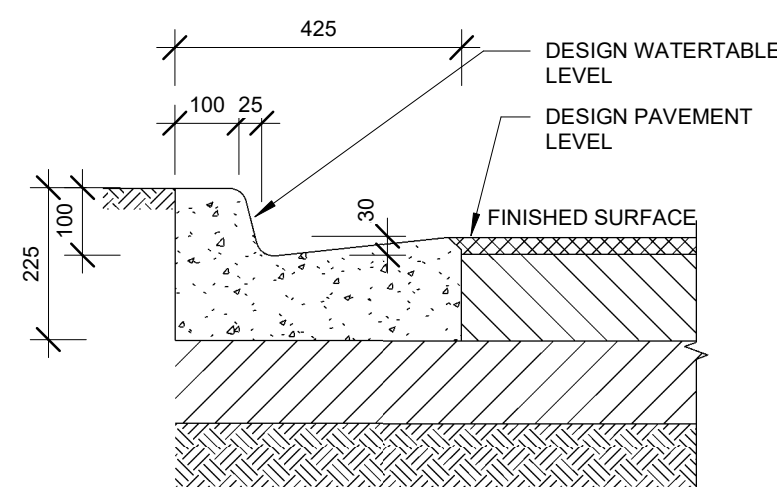
100 HIGH KERB & WATERTABLE Scale 1:10
