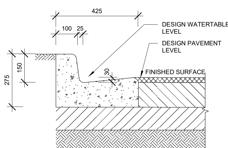
150 HIGH KERB & WATERTABLE Scale 1:10
