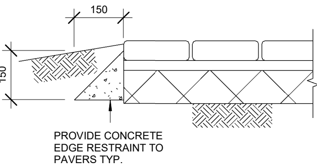
MASONRY PAVEMENT EDGE DETAIL Scale 1:10
