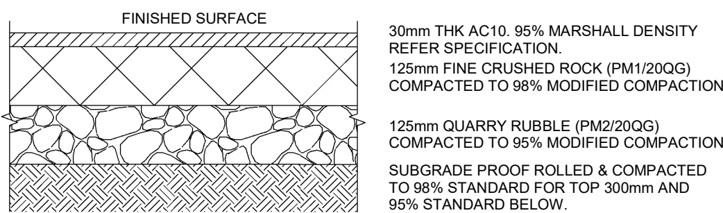
ASHALT PAVEMENT - LIGHT DUTY (BASKETBALL COURT) Scale 1:10
