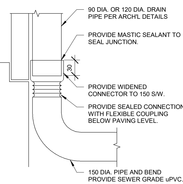
NEW DOWNPIPE CONNECTION DETAIL Scale 1:10
