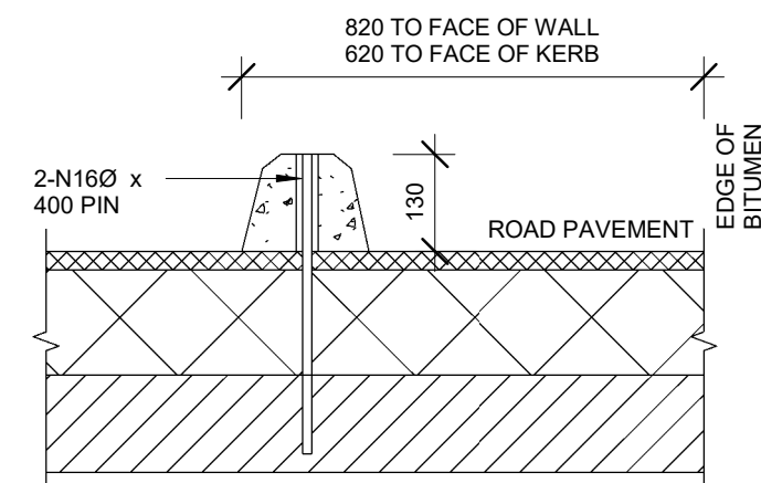
CONCRETE WHEEL STOP Scale 1:10
