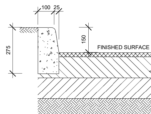
150 HIGH KERB Scale 1:10
