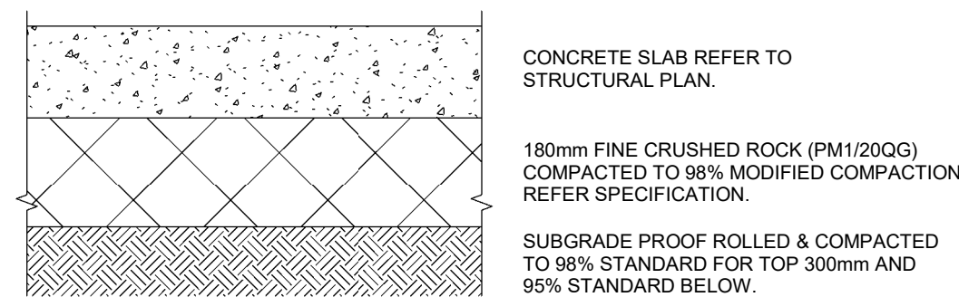
CONCRETE PAVEMENT - MEDIUM DUTY (CARPARK PAVING) Scale 1:10
