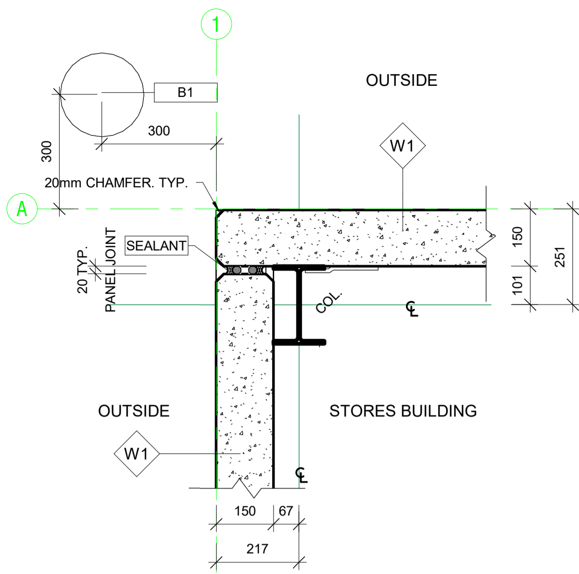
NOTE: TYPICAL CONC DADO PANEL DETAIL UP TO 2400 AFFL PD.01 Plan Detail PD.01 1:10
