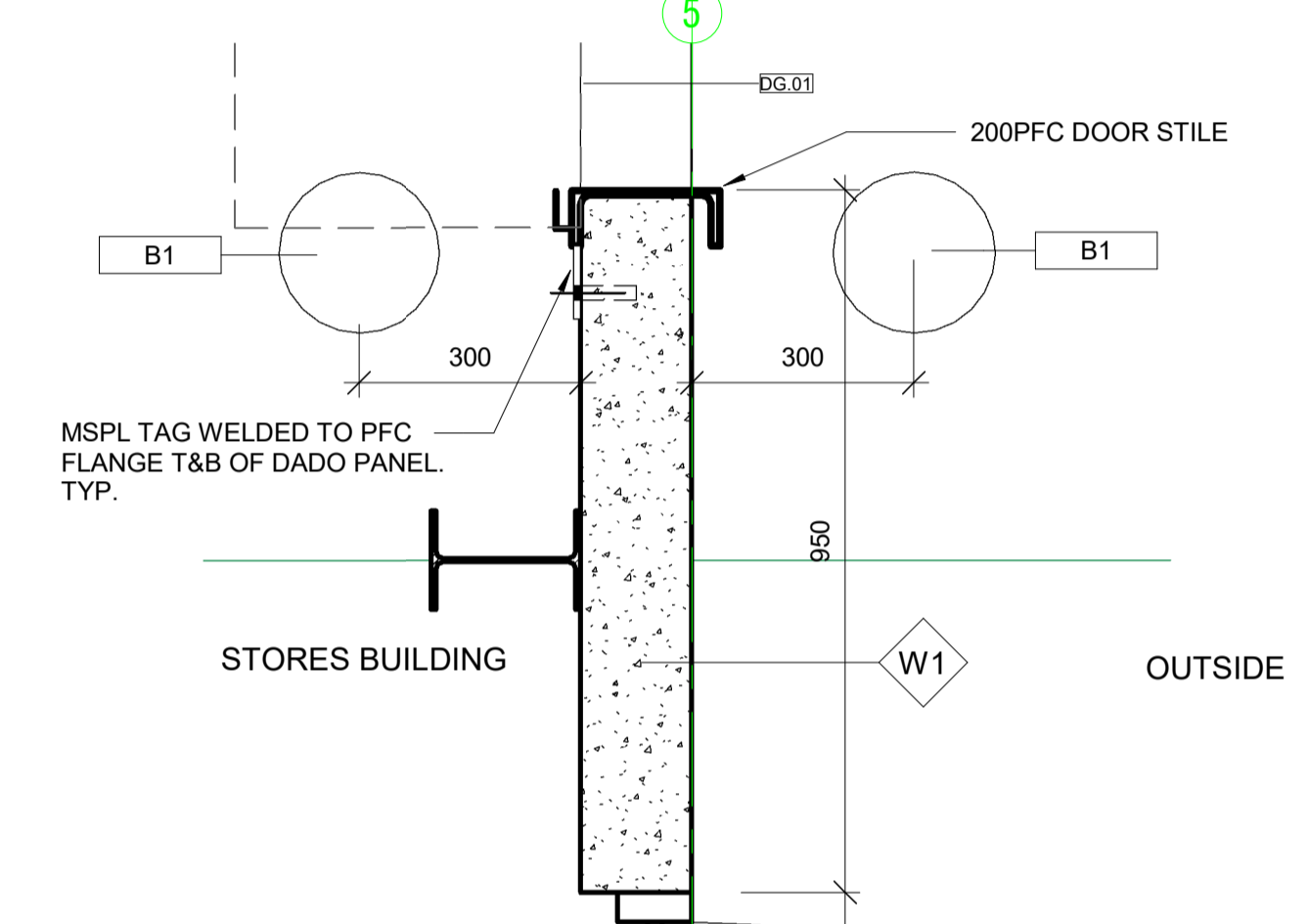
PD.03 Plan Detail PD.03 1:10
