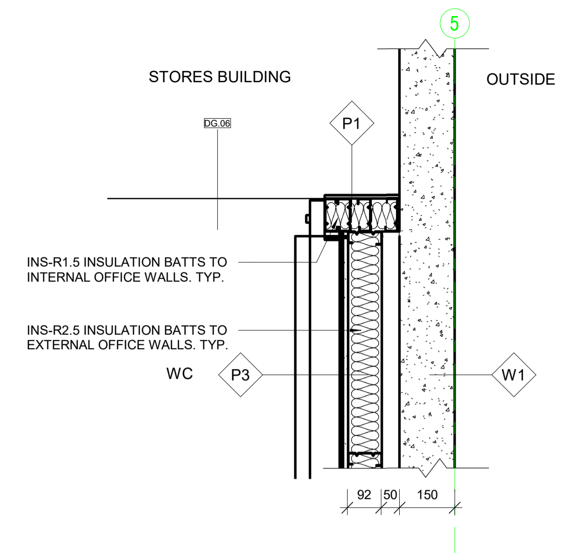
PD.05 Plan Detail PD.05 1:10
