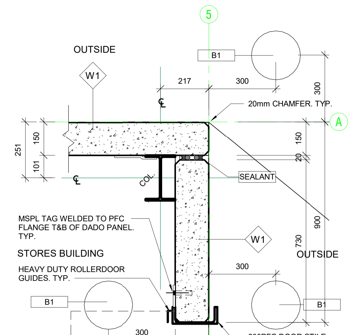
PD.03 Plan Detail PD.03 1:10
