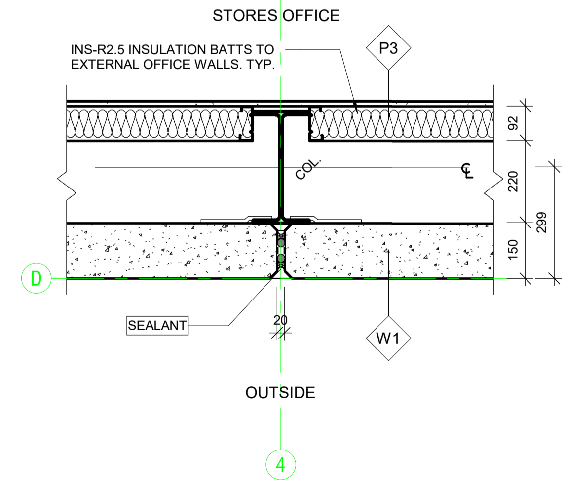
PD.04 Plan Detail PD.04 1:10
