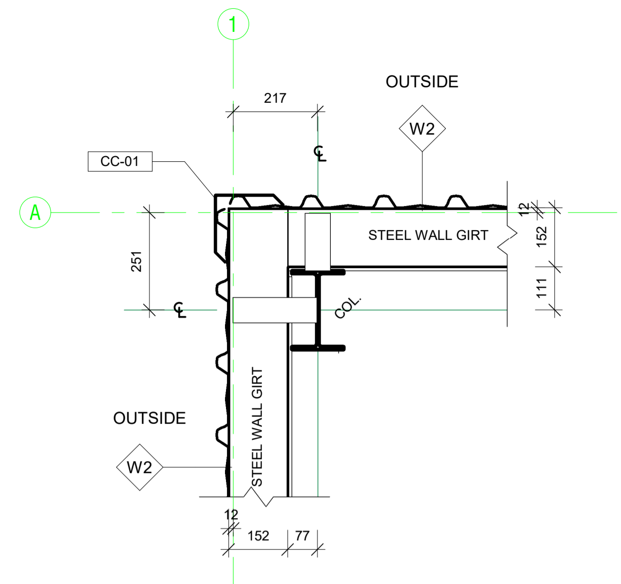
NOTE: TYPICAL DETAIL ABOVE 2400 AFFL PD.02 Plan Detail PD.02 1:10
