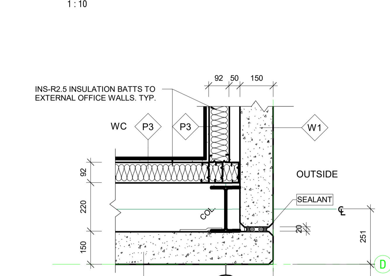
PD.05 Plan Detail PD.05 1:10
